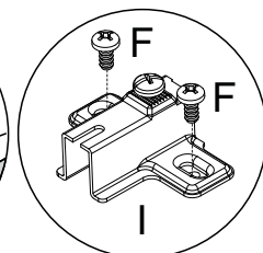
Detalhe 3 Detail/Detaille
